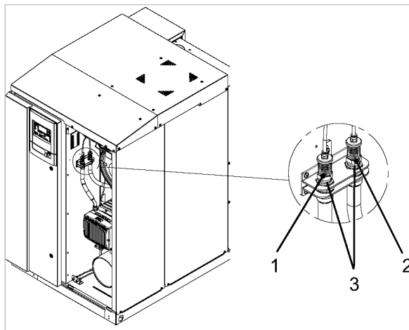
Fig. 28 Replenishing lubricating oil
