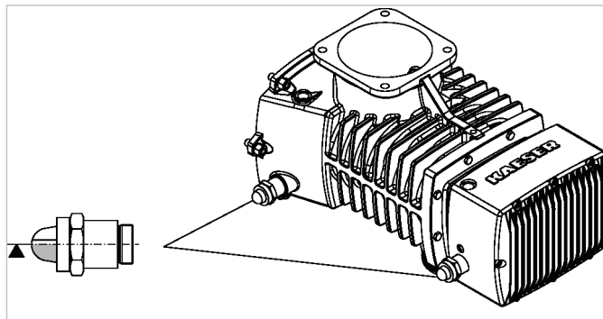
Fig. 27 Checking the lubricating oil level
