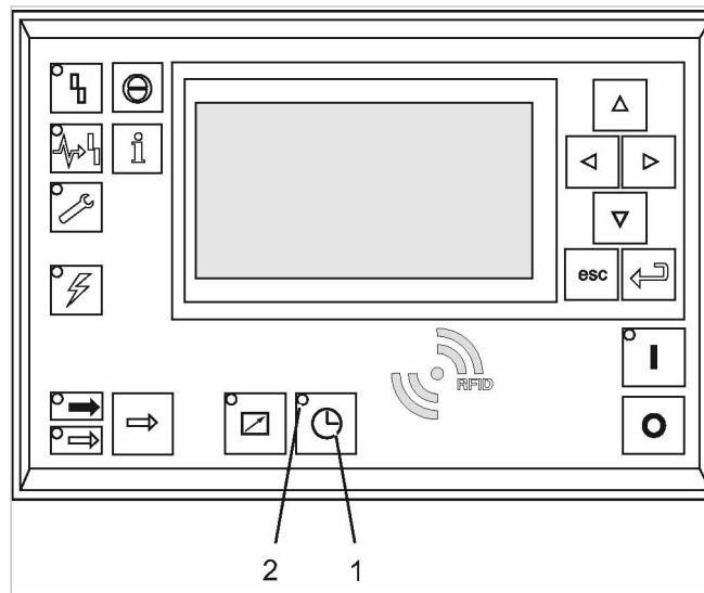
Fig. 23 Switching on and off with the clock (timer)
